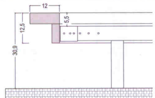
CROSS BAR SUPPORTS
